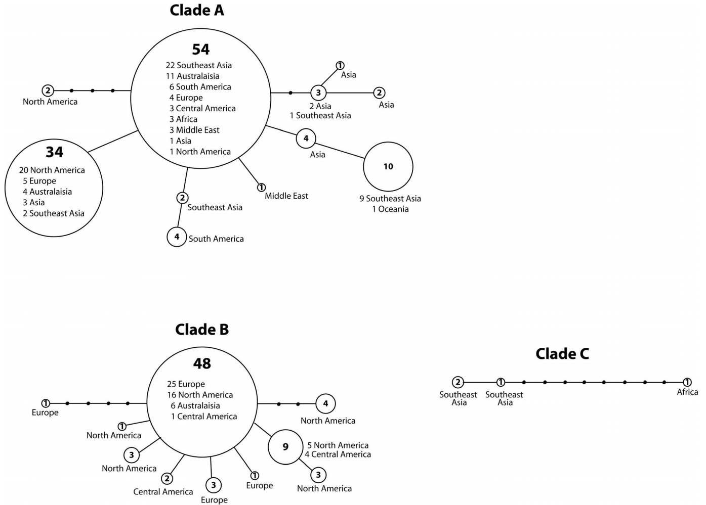
FIG. 2. Statistical parsimony networks for mitochondrial COI Clades A, B, and C. Each connection represents a single mutational step with inferred haplotypes represented by small black circles. Observed haplotypes are shown as large circles with haplotype frequency indicated within the circles. For each haplotype, geographic distribution and frequency is indicated.
