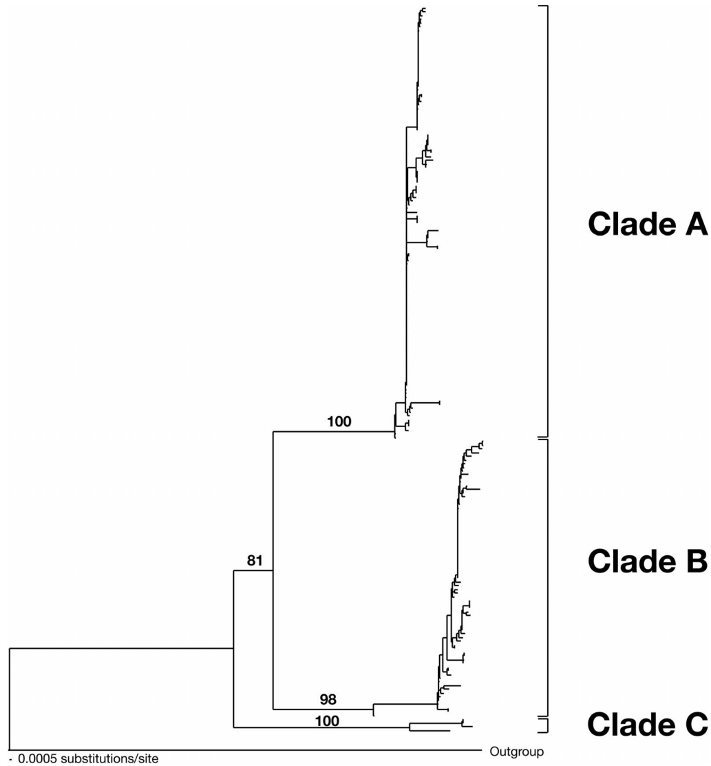
FIG. 1. NJ phylogram resulting from analysis of the double-stranded mitochondrial COI data available on GenBank and collected as part of this study. Bootstrap support values greater than 75 (based on 1,000 NJ bootstrap replicates) are located above the nodes. Mitochondrial clade memberships are indicated to the right of each tree. Head and body lice belonging to Clade A are distributed worldwide; head lice belonging to Clade B are restricted to North and Central America, Europe, and Australia; and head lice belonging to Clade C are restricted to Ethiopia and Nepal.
